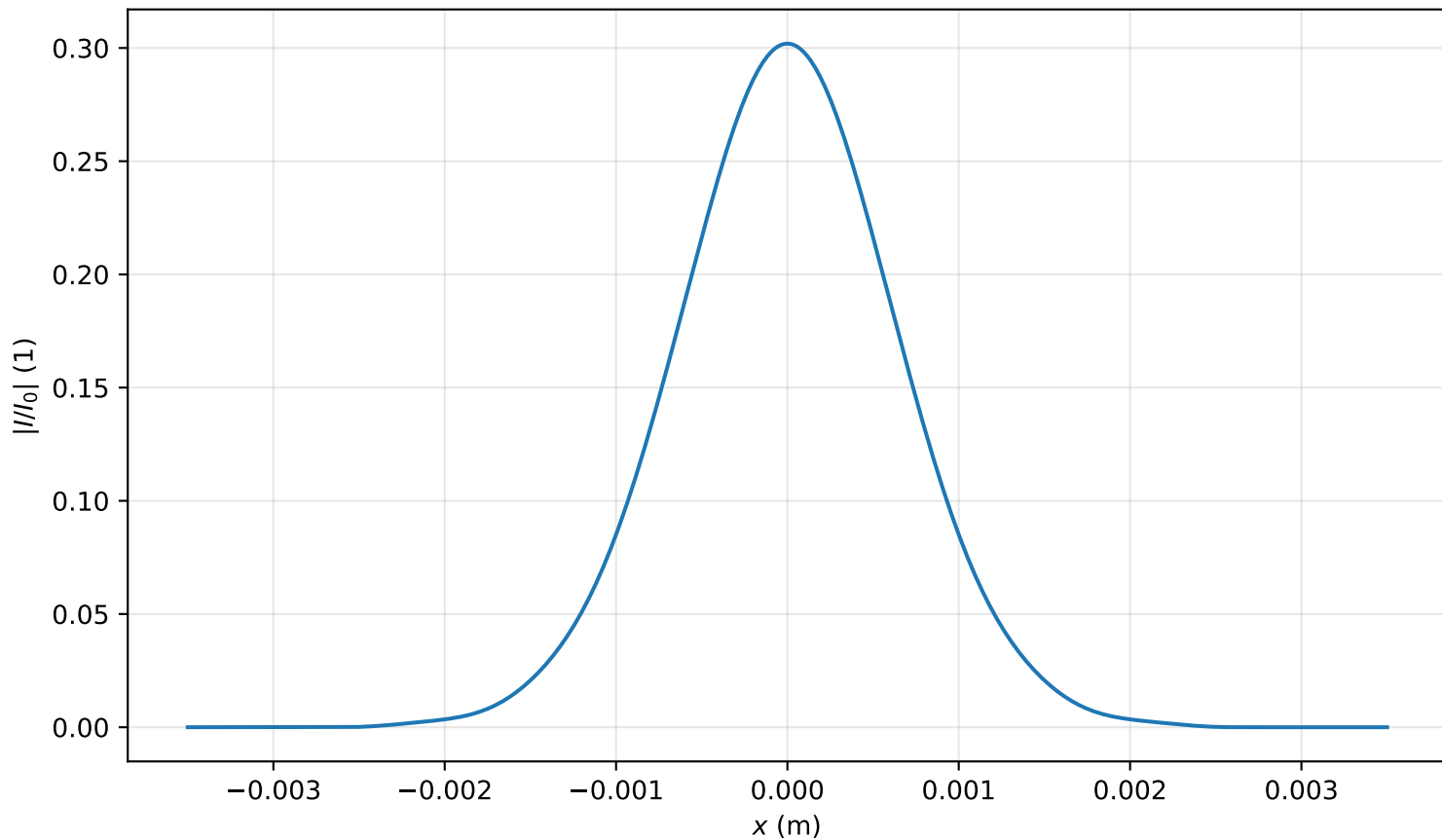
Intensity profile I(x, y = 0, z = 3.821m)/I_0 , P_{in}=0.3P_{cr} , artificial time
